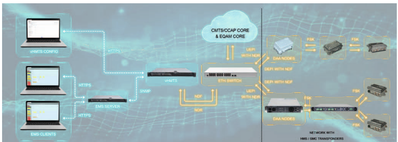
Schematic operation of the vHMTS and its integration into the narrowband monitoring system
