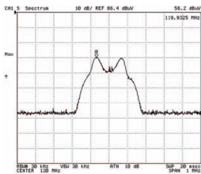
Generated FSK signal at the output of the RPD
