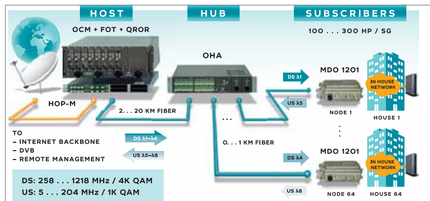
The FTTB solution from Comtech
